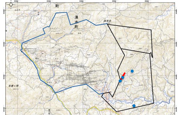
Figure 3: Plan map showing the outline of the Yamagano Mining Lease (blue, optioned by Irving), the outline of the western part of the East Yamagano claim block (black), the traces of Yamagano underground mine workings (gray) and the trace of hole 23SY-001 (red).
